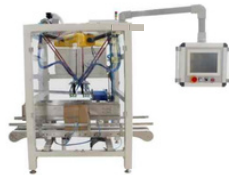
ADR-1 Delta robot hand loading machine 蜘蛛手开瓶机器人装箱 Vision accuracy/视觉精度: \pm 0.5\text{mm} Positioning accuracy/定位精度: 0.1\text{mm} Dimension/直径: 880 \times 1130\text{mm} Work speed/最大速度: 15 \sim 25\text{carton/min} Machine size/外形尺寸: 950 \times 1050\text{mm}
