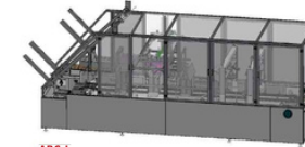
ABC-1 Cardboard Carton Erector 纸板裹包式装箱机 Suitable Case/适用纸箱: 550 \times L \times W \times H100 \sim 1000\text{mm} Work speed/箱速: 15 \sim 18\text{carton/min} Machine size/机身尺寸: L5130 \times W2600 \times H1800\text{mm} Production ability/生产能力: L460 \times W280 \times H350
