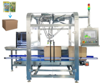
蜘蛛手装箱机 Spider Pick-Put Carton Packing Machine
